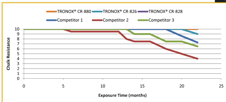
Coil Coating Top Coat Allunga* 45° North
