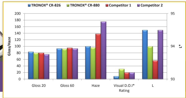
Automotive Topcoat Allunga 5° North
