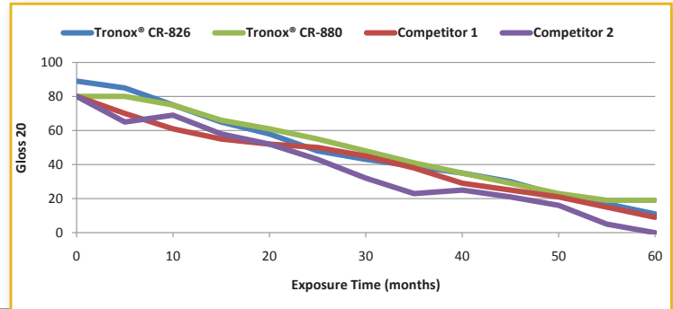
Automotive Solid Colour Exposure Allunga 5° North
