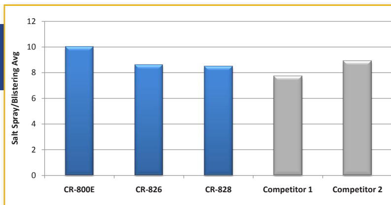
Salt Spray/Blistering Averages
