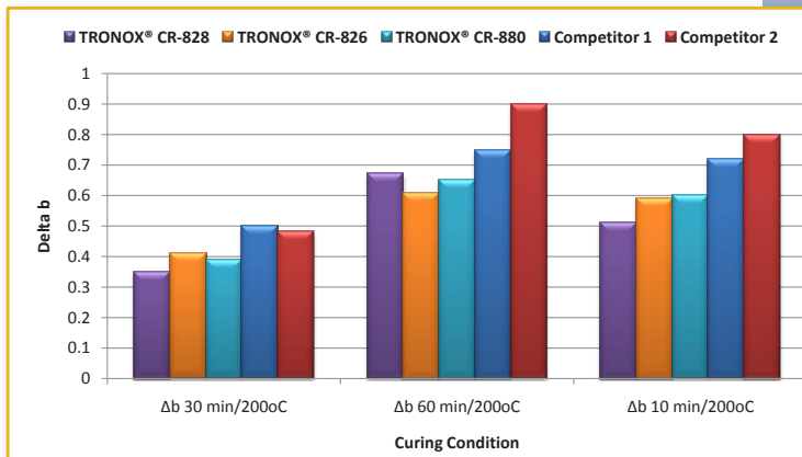
Overbake Comparison in Primid System
