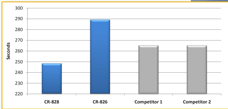
Overbake Comparison in Primid System
